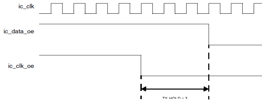
Figure 26-3: Timing Diagram for I2C Master Mode TX_HOLD = 3
