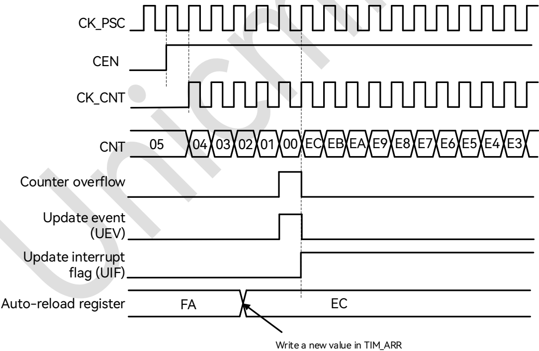
Figure 19-10: Down-counting Waveform Diagram, Internal Clock Divided by 2
