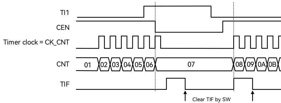
Figure 19-34: Timing Diagram in Gated Mode
