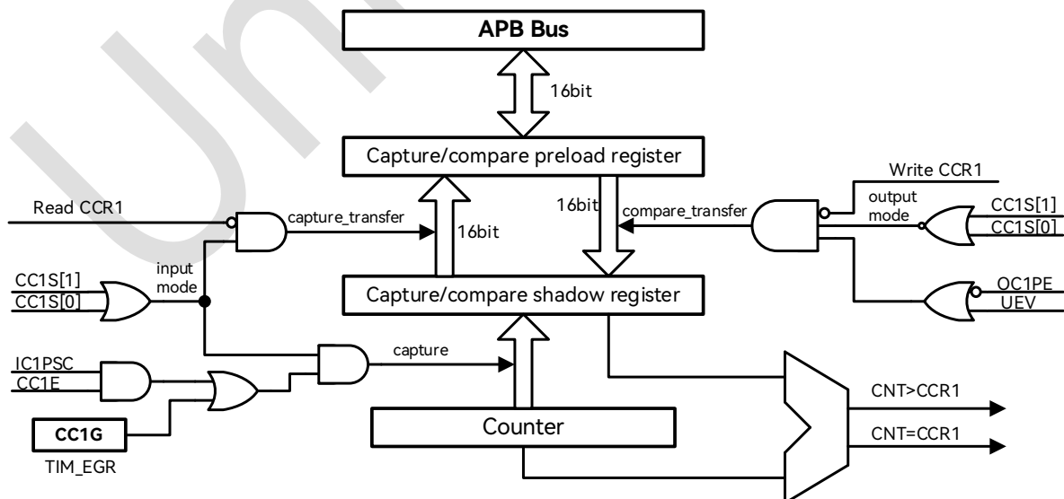
Figure 18-24: Capture/Compare Channel 1 Main Circuit
