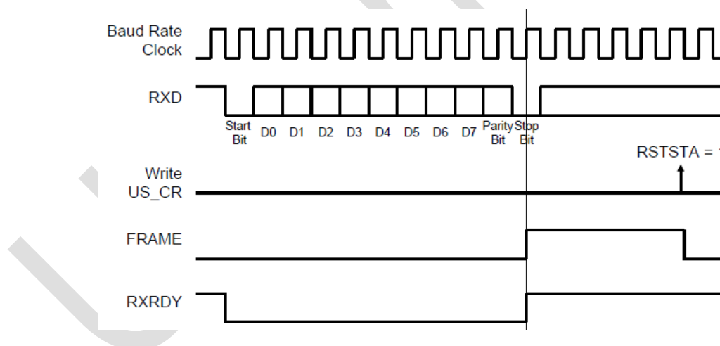
Figure 30-19: Timing Diagram of Frame Error Status
