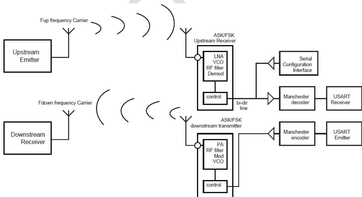
Figure 30-12: Manchester Encoded Character RF Transmission
