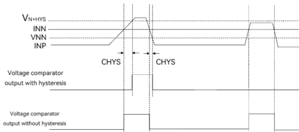
Figure 38-3: Voltage Comparison Function with Hysteresis
