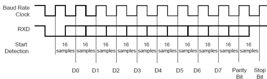
Figure 30-8: Character Reception
