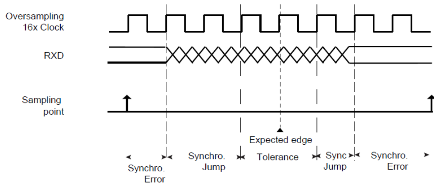
Figure 30-6: Bit Synchronization Diagram
