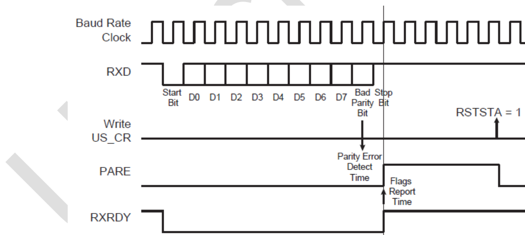
Figure 30-17: Parity Error Timing Diagram
