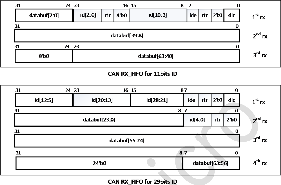
Figure 25-2: RXBUF Register Data Format
