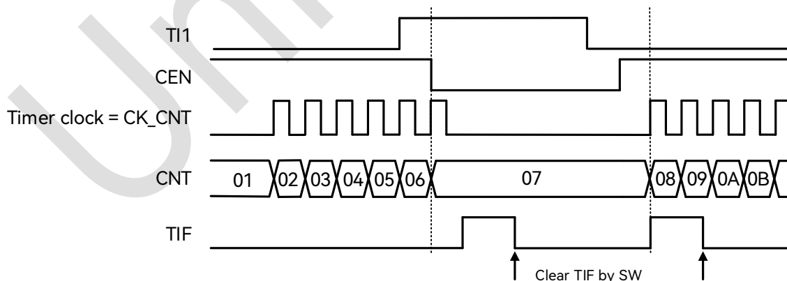
Figure 18-40: Timing Diagram in Gated Mode
