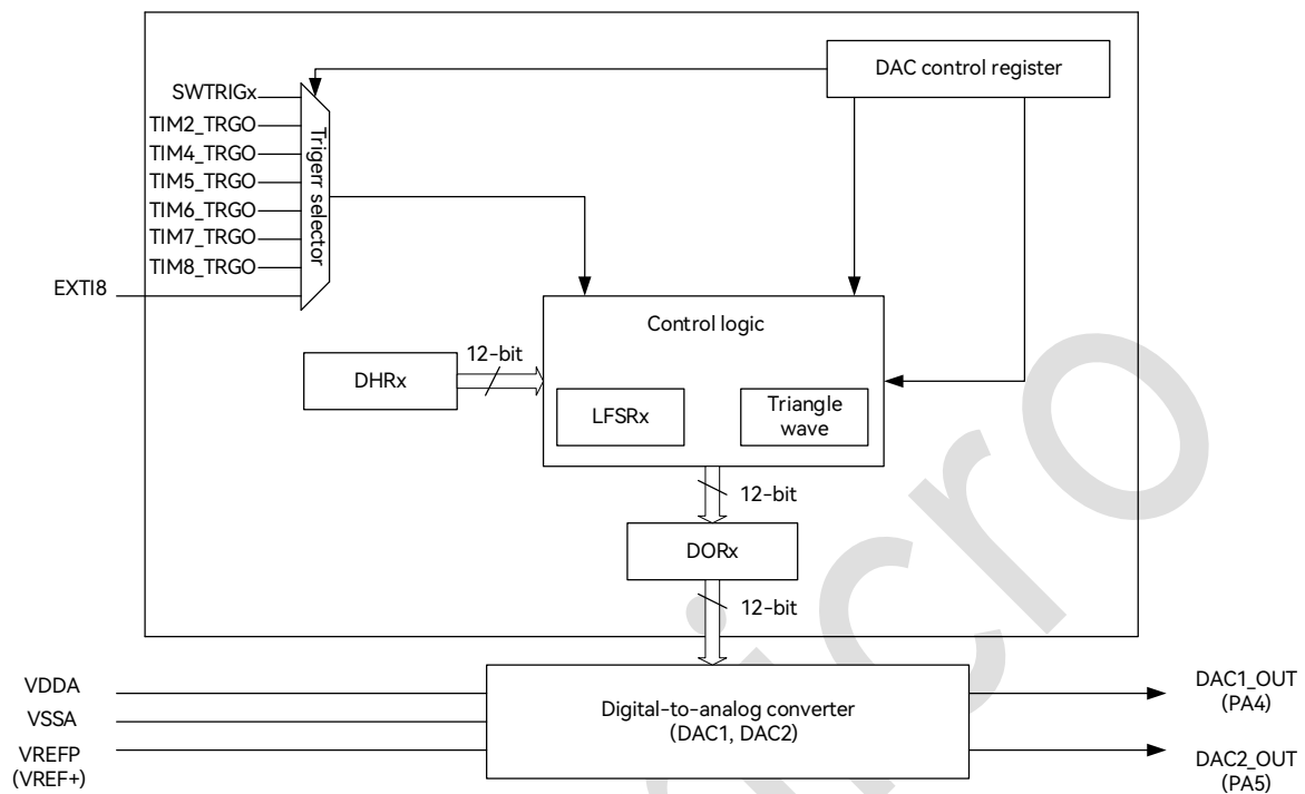
Figure 37-1: DAC System Block Diagram
