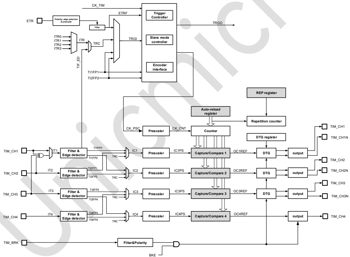
Figure 18-1: TIM1 & TIM8 System Block Diagram
