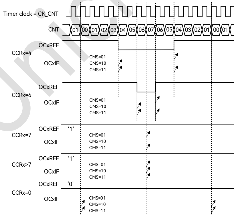
Figure 19-29: Center-aligned PWM Waveform (ARR = 7)
