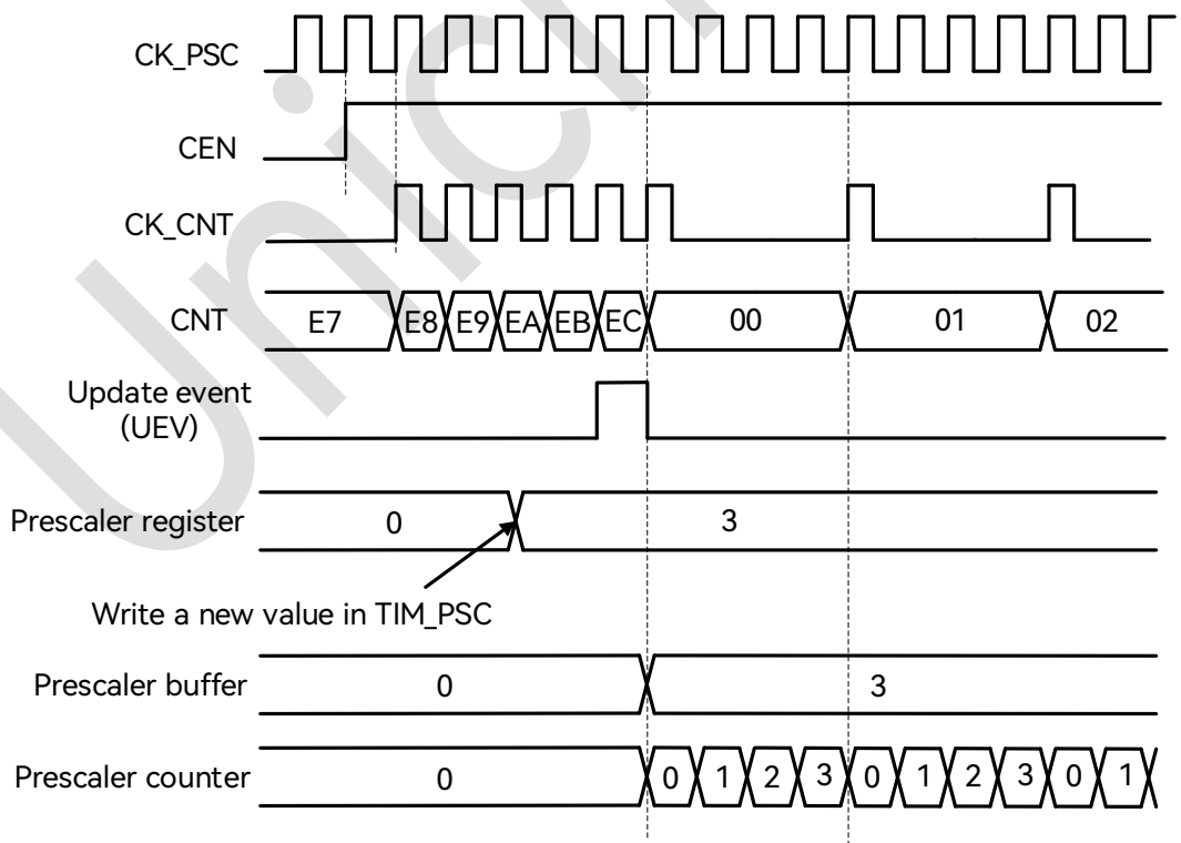
Figure 18-3: Counter Timing Diagram with Prescaler Division Changing from 1 to 4
