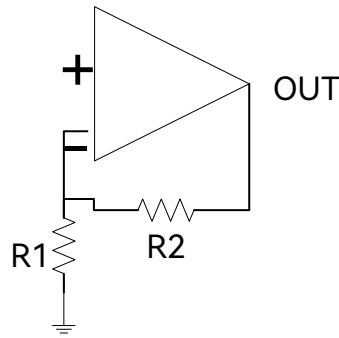
Figure 39-1: External Amplifier Circuit Connection Diagram
