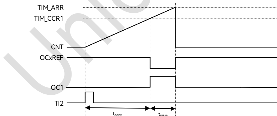
Figure 19-30: Timing Diagram of One-pulse Mode
