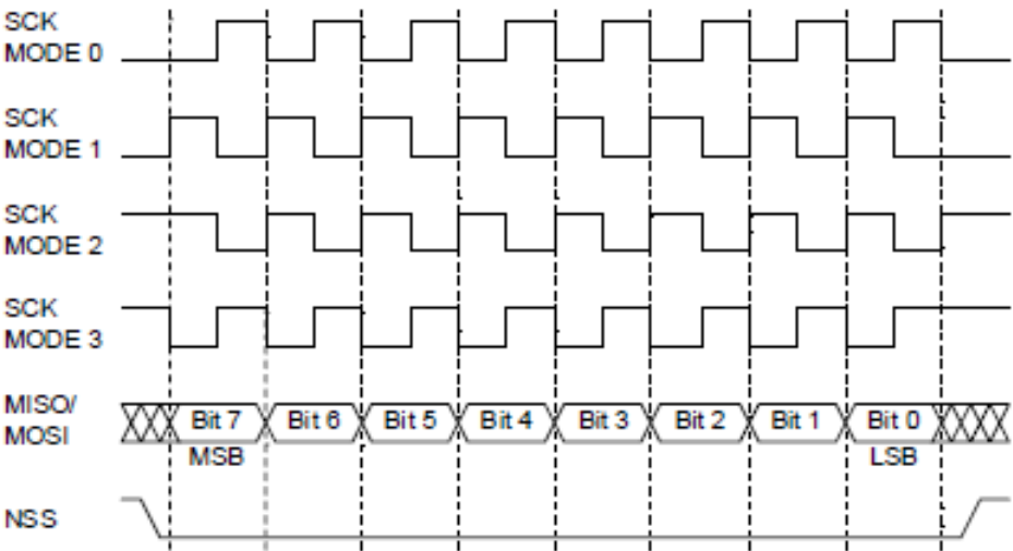
Figure 31-4: Transmission Timing Diagram of SPI in Different Modes in Motorola Mode
