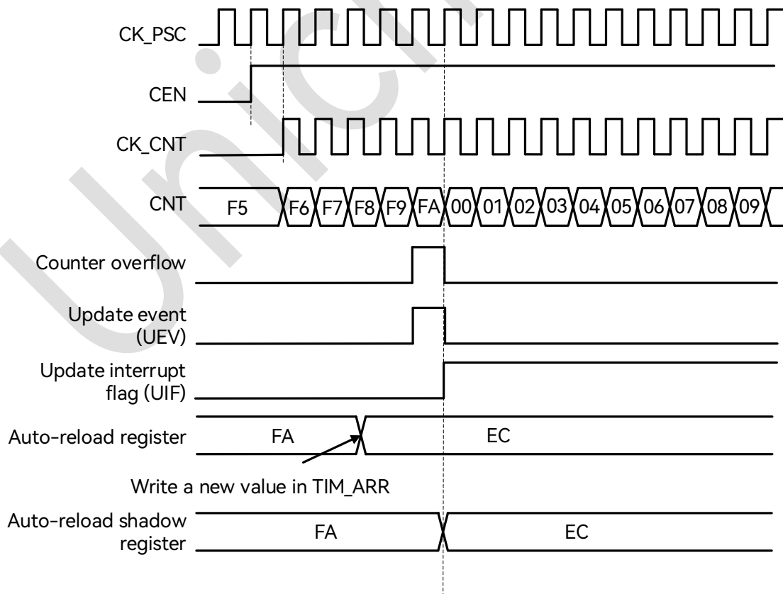
Figure 20-6: Counter Timing Diagram, Update Event when ARPE = 1 (TIM_ARR Preloaded)
