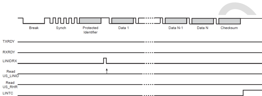
Figure 30-40: Slave Node Configuration, NACT = IGNORE
