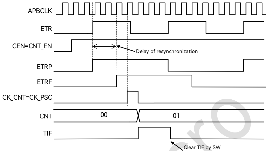
Figure 18-21: Timing 1 Diagram in External Clock Source Mode 2
