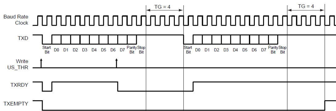
Figure 30-18: Timing Diagram of Time Protection Operation
