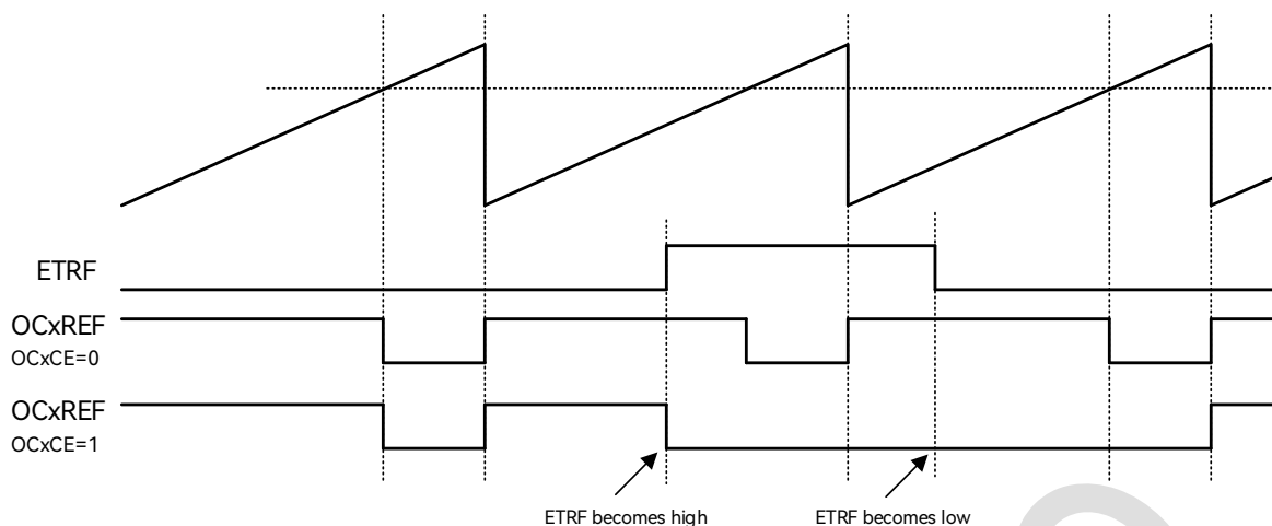
Figure 18-37: Timing Diagram of ETR Signal Clearing OCxREF of TIM
