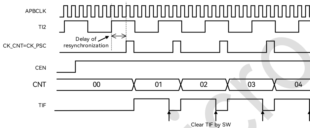
Figure 19-18: Timing Diagram in External Clock Source Mode 1
