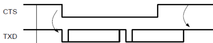
Figure 30-23: Transmitter Operation Behavior When Hardware Handshake is Enabled
