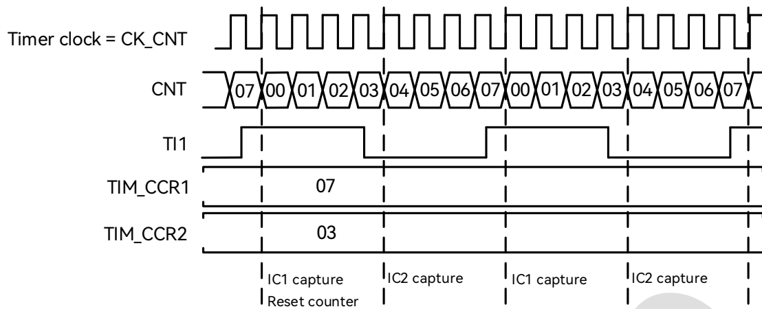
Figure 18-27: PWM Input Capture Mode Timing Diagram
