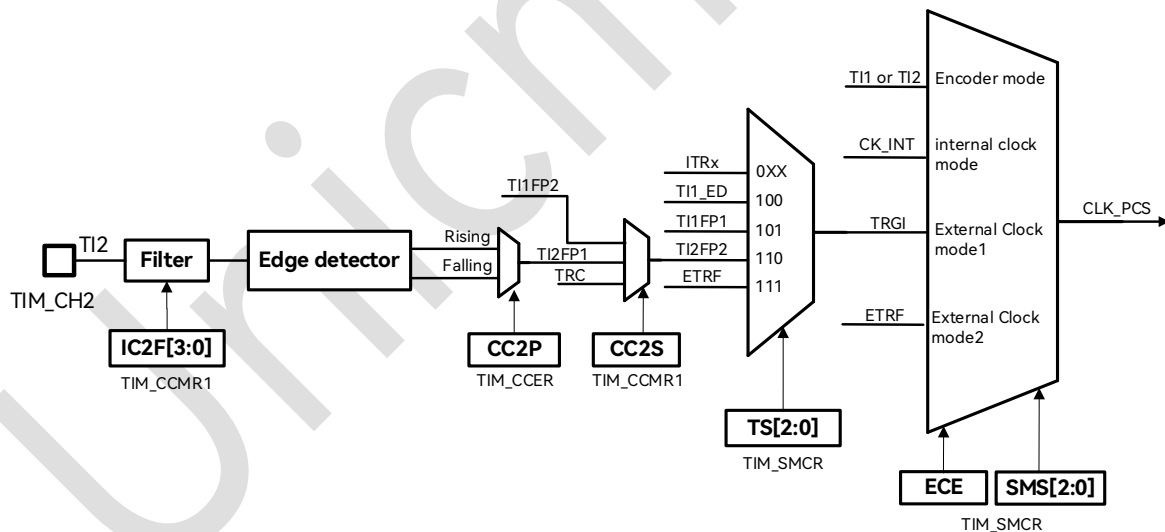
Figure 19-16: Example of External Clock Connection
