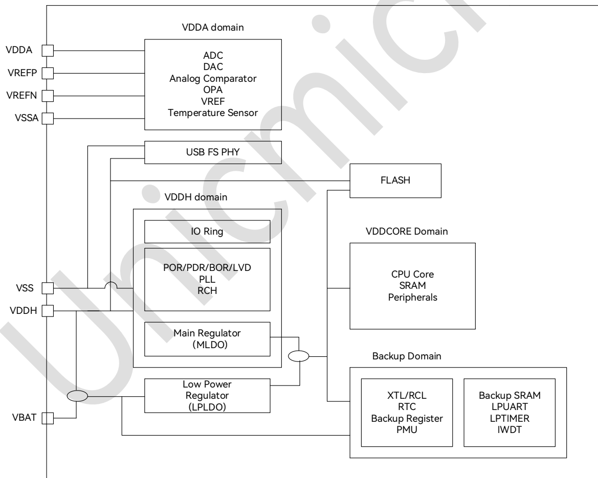
Figure 5-1: System Power Supply Scheme
