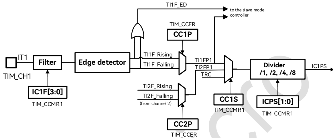
Figure 18-23: Capture/Compare Channel (Channel 1 Input Stage)
