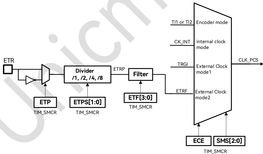
Figure 18-20: External Trigger Input Block Diagram
