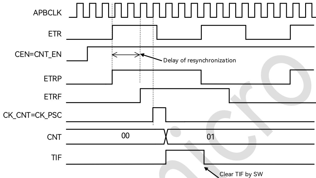
Figure 19-20: Timing 1 Diagram in External Clock Source Mode 2
