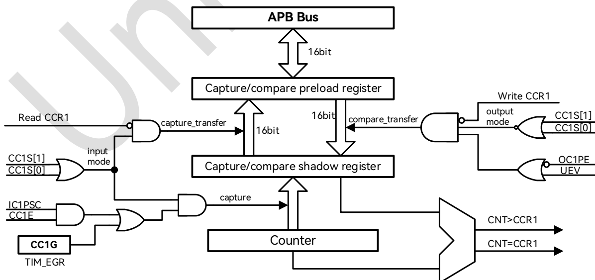
Figure 19-23: Capture/Compare Channel 1 Main Circuit
