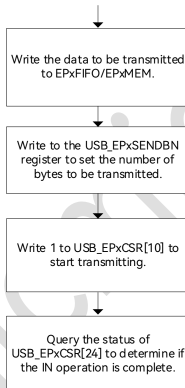
Figure 35-2: USB Endpoint In Transfer Flowchart
