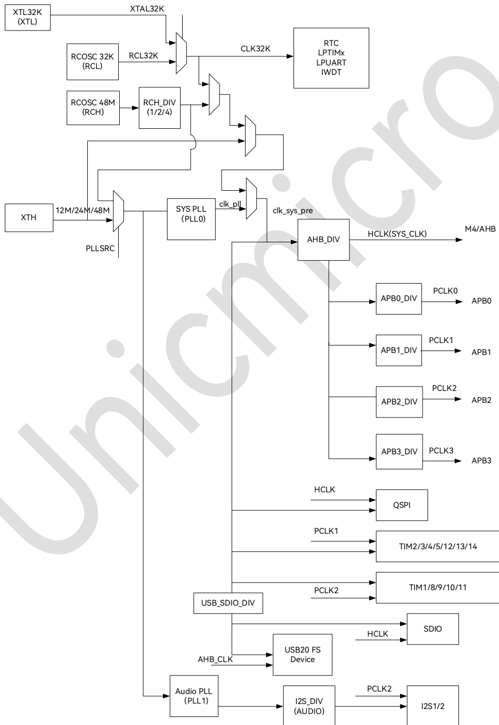
Figure 6-1: Clock Logic
