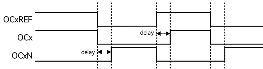
Figure 18-31: Waveform of Complementary Output with Dead-time Insertion
