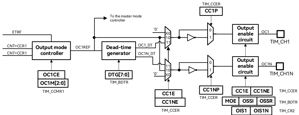
Figure 19-24: Output Stage of Capture/Compare Channel (Channels 1-3)
