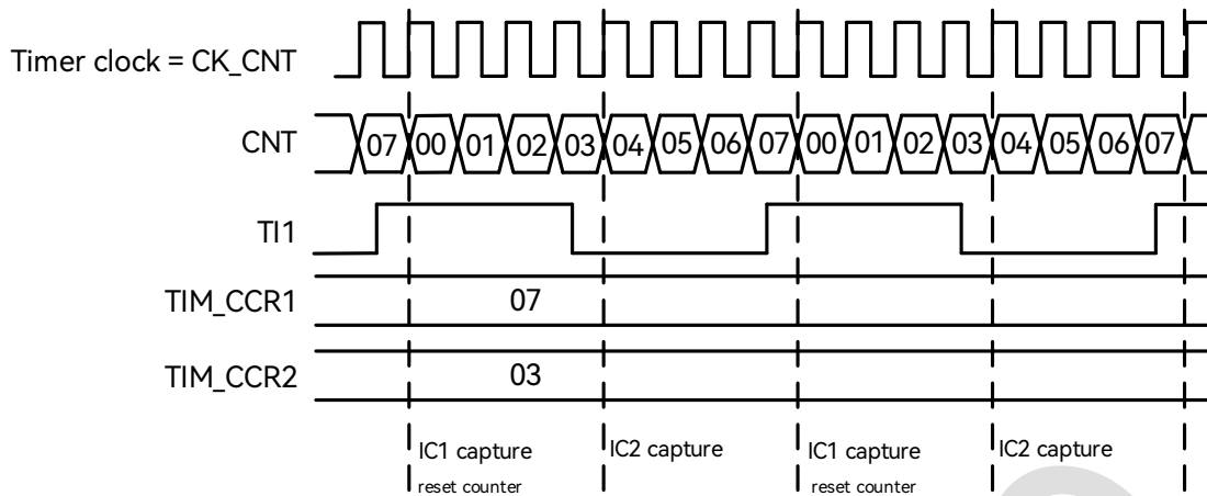
Figure 19-26: PWM Input Capture Mode Timing Diagram
