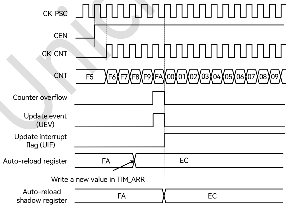
Figure 19-7: Counter Timing Diagram, Update Event when ARPE = 1 (TIM_ARR Preloaded)
