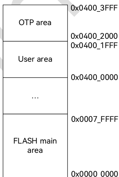
Figure 4-1: EFC Memory Address Mapping
