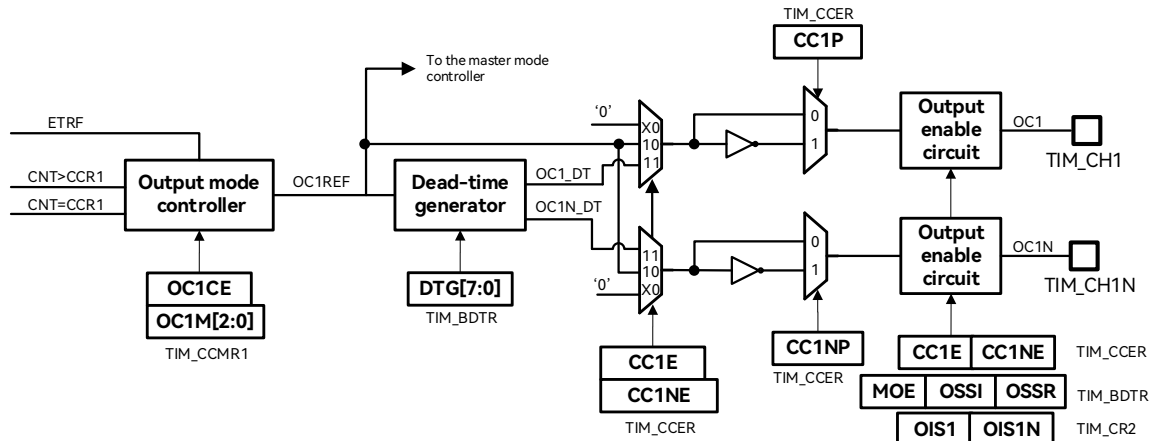
Figure 18-25: Output Stage of Capture/Compare Channel (Channels 1-3)
