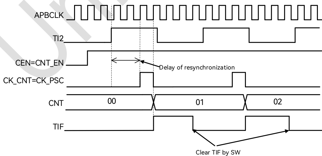
Figure 18-18: Timing Diagram in External Clock Source Mode 1
