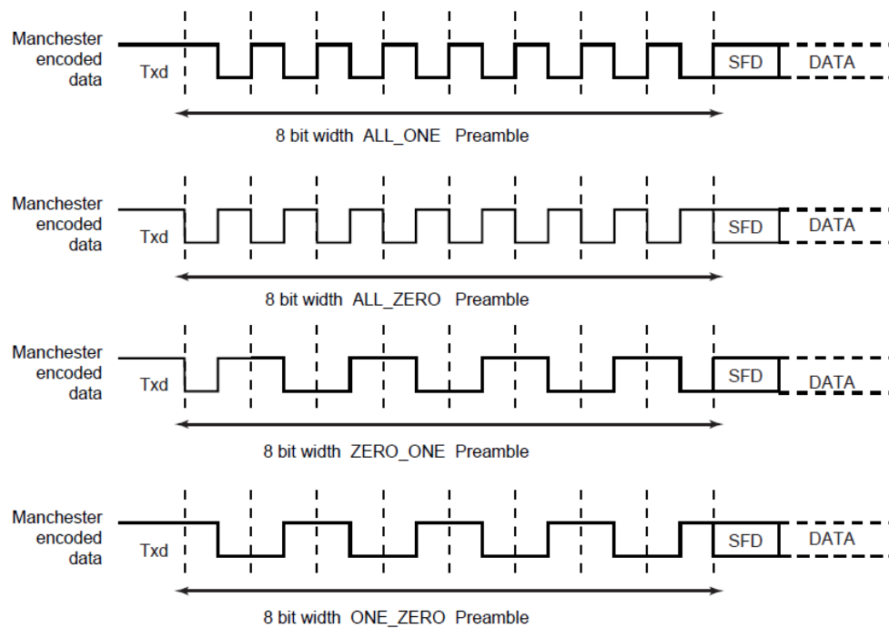
Figure 30-4: Preamble Signal Mode
