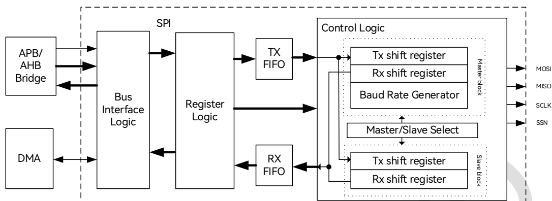
Figure 31-1: SPI Module Block Diagram
