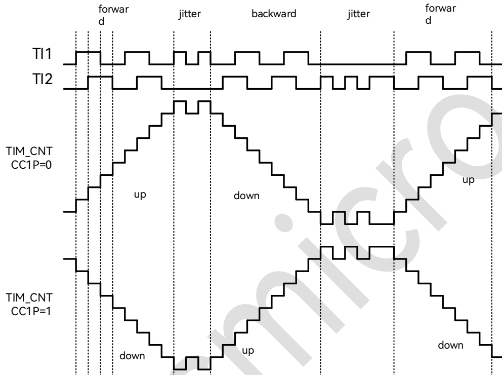
Figure 19-32: Example of Counter Operation in Encoder Interface Mode
