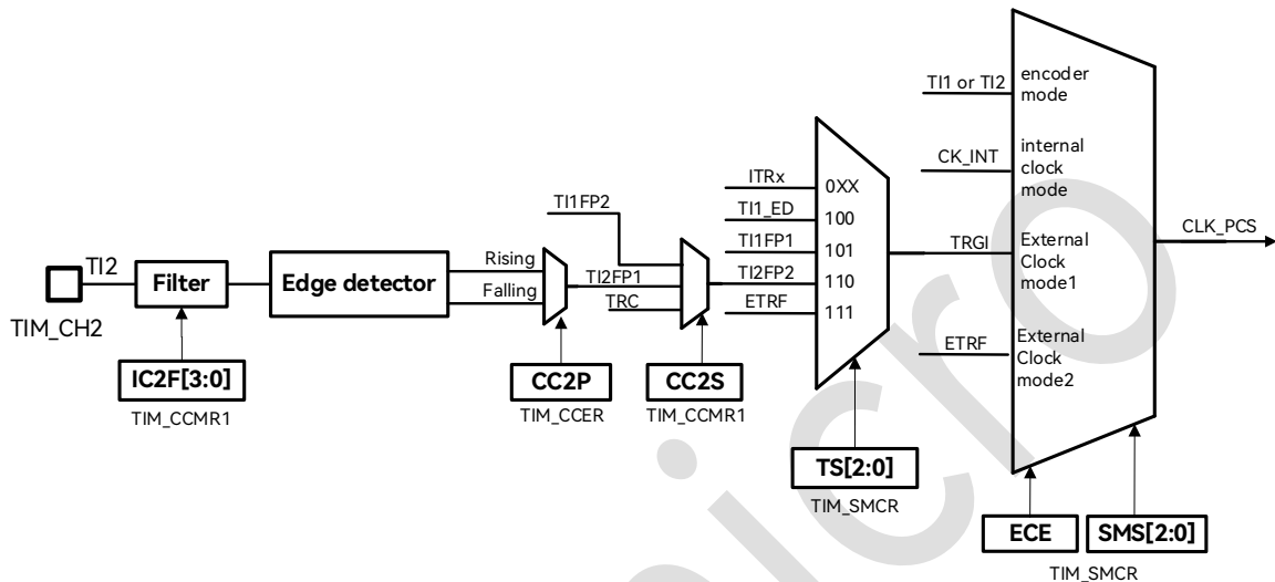
Figure 18-17: External Clock Connection Diagram
