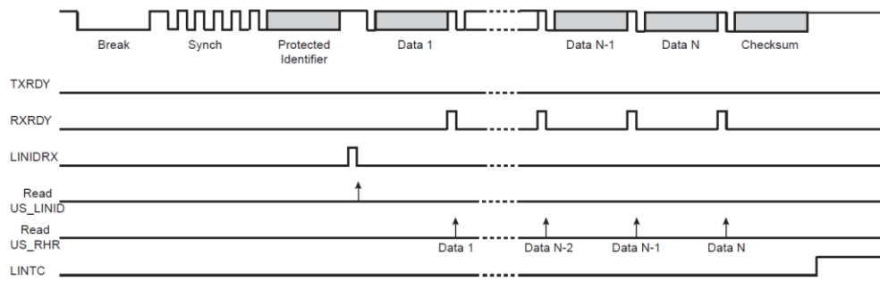
Figure 30-39: Slave Node Configuration, NACT = SUBSCRIBE
