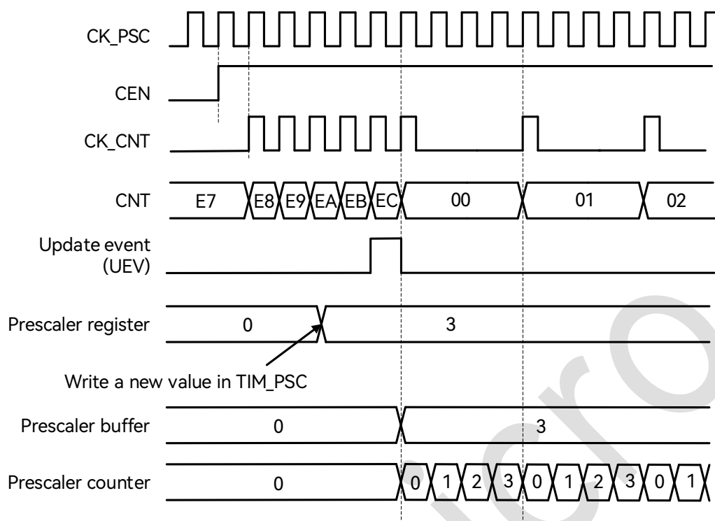
Figure 19-3: Counter Timing Diagram with Prescaler Division Changing from 1 to 4
