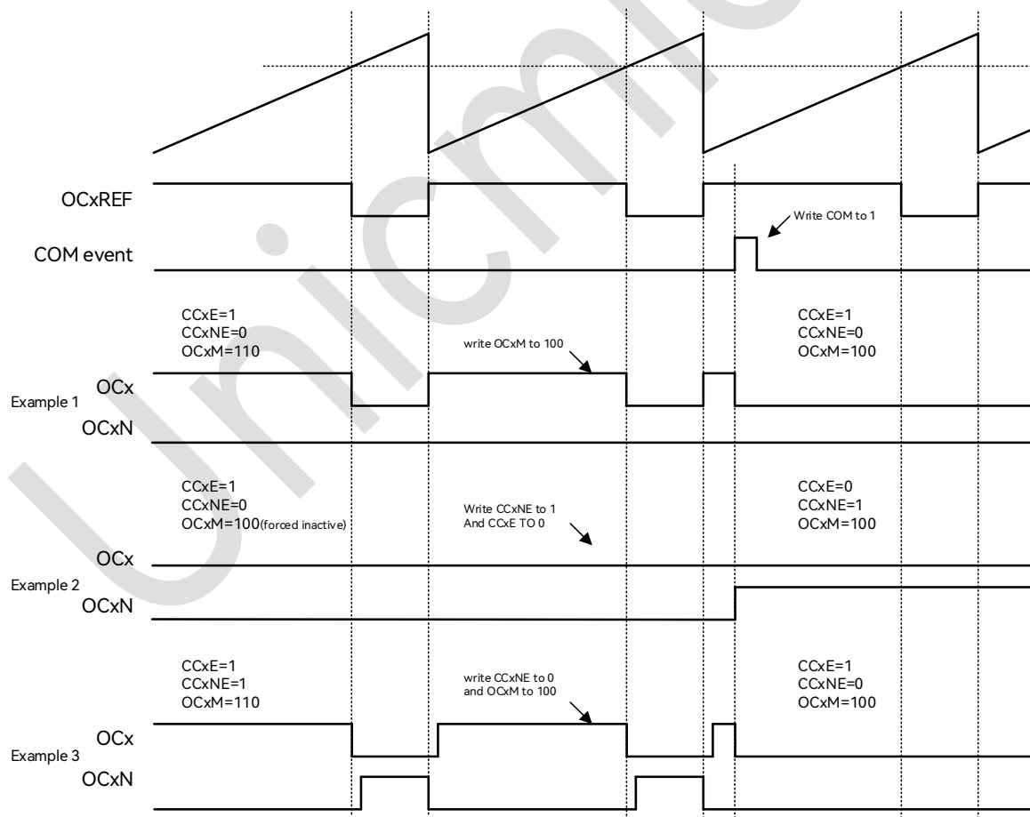
Figure 18-35: 6-step PWM Generation, COM Example (OSSR = 1)
