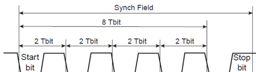
Figure 30-31: Sync Field
