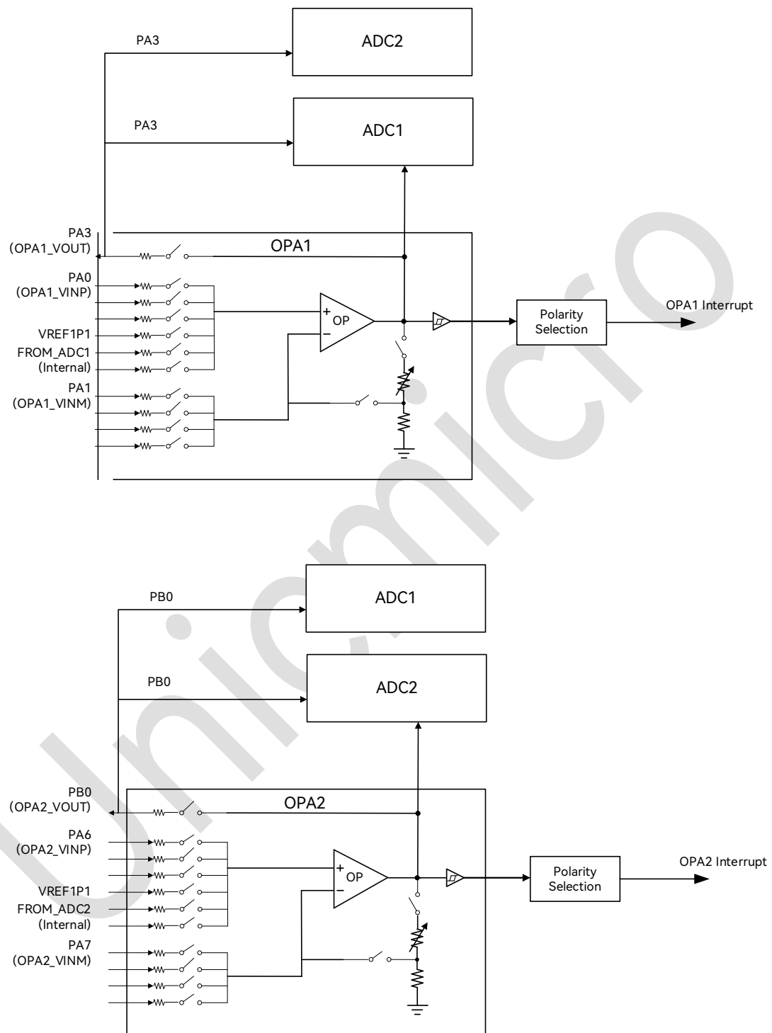
Figure 39-1: OPA System Block Diagram
