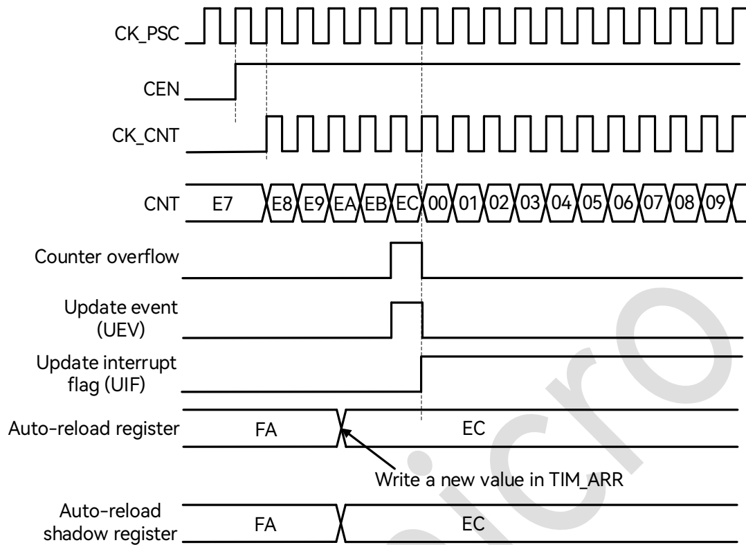
Figure 19-6: Counter Timing Diagram, Update Event when ARPE = 0 (TIM_ARR not Preloaded)
