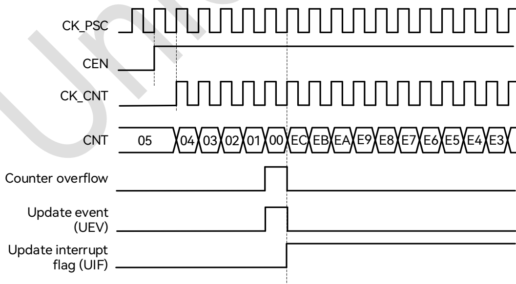
Figure 19-8: Down-counting Waveform Diagram, Internal Clock not Divided
