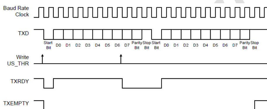
Figure 30-2: USART Transmitter Status
