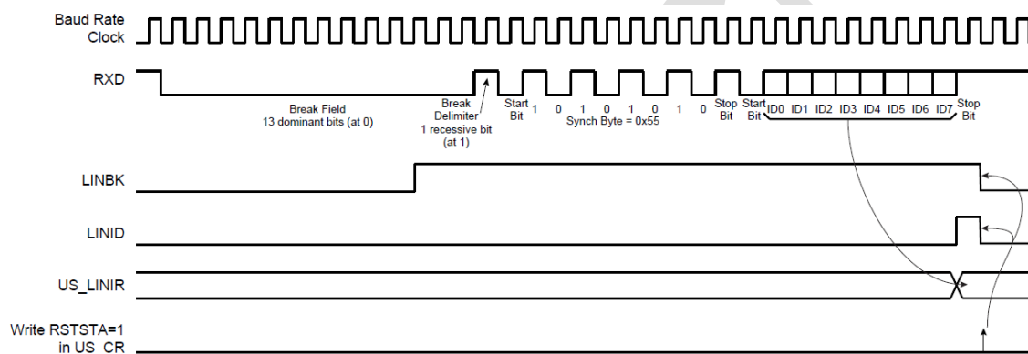
Figure 30-30: Message Reception
