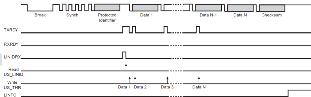
Figure 30-38: Slave Node Configuration, NACT = PUBLISH
