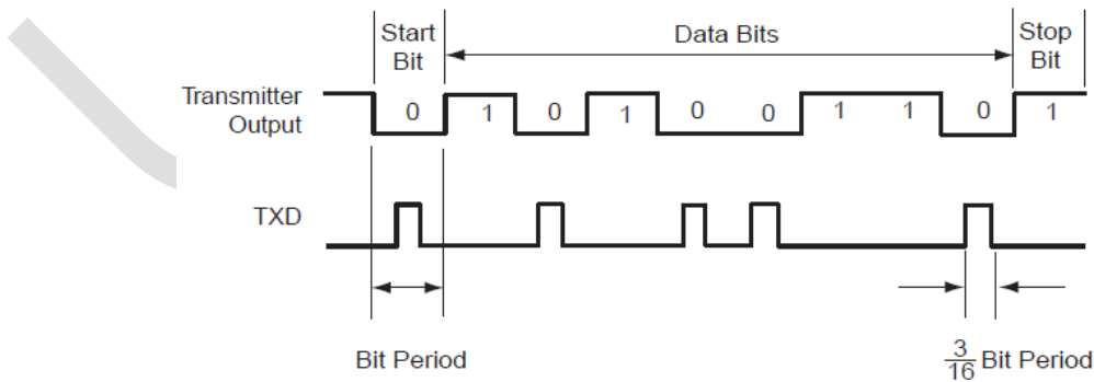
Figure 30-25: IrDA Modulation
