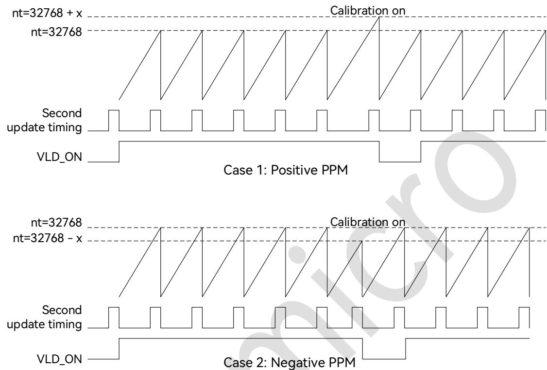
Figure 24-2: Oscillator Calibration
