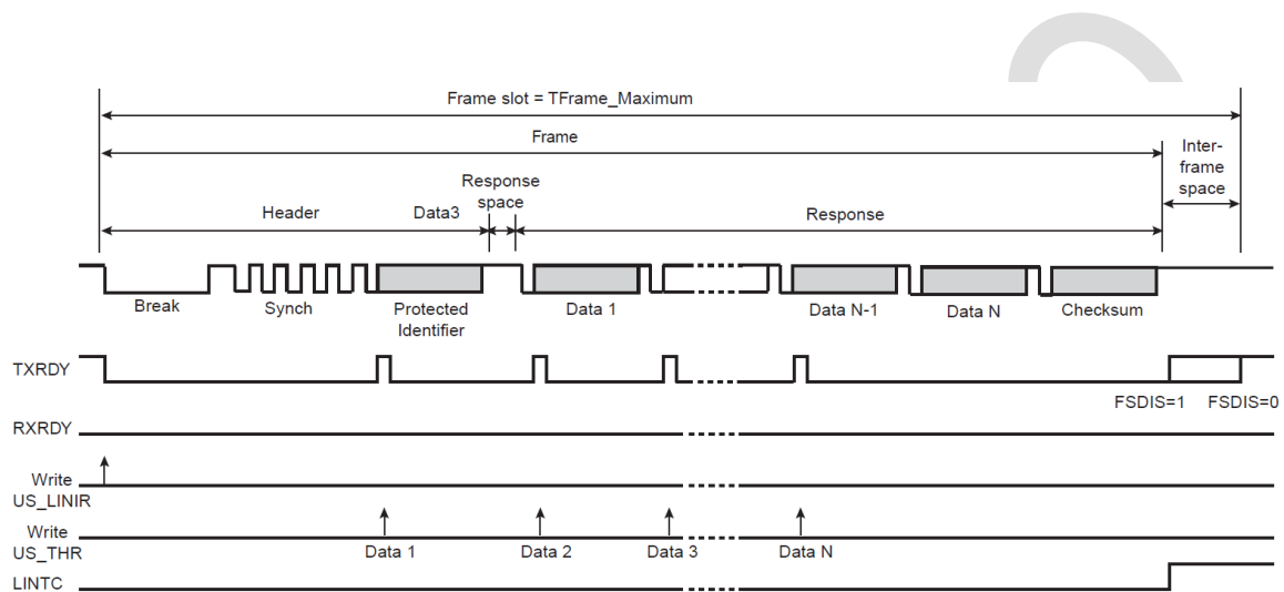
Figure 30-35: Master Node Configuration, NACT = PUBLISH
