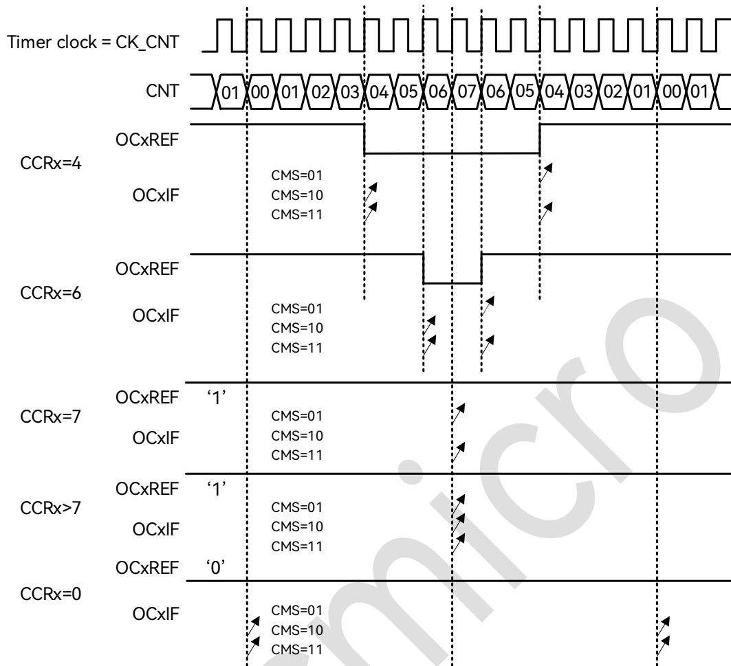
Figure 18-30: Center-aligned PWM Waveform (ARR = 7)
