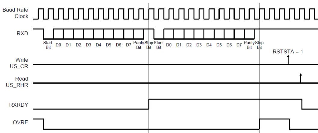
Figure 30-16: Receiver Status
