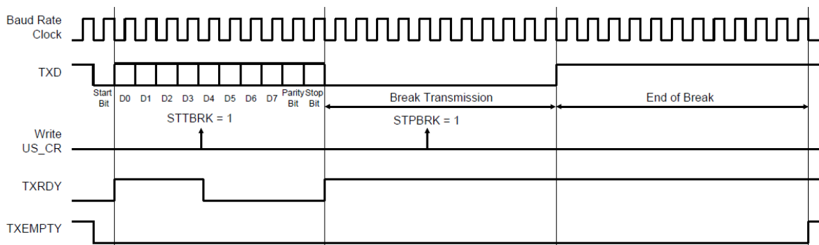
Figure 30-20: Transmission of Break
