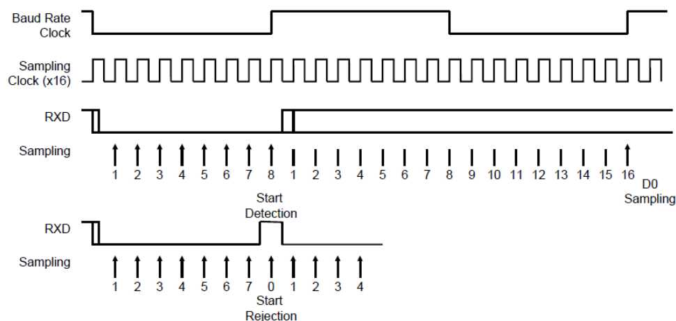
Figure 30-7: Asynchronous Start Bit Detection
