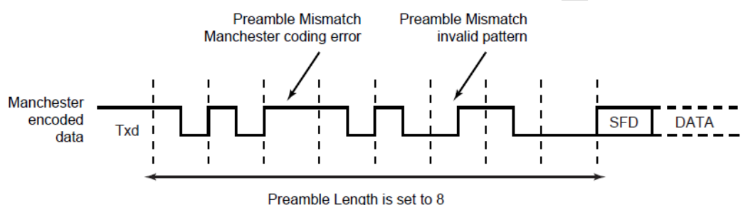
Figure 30-10 : Preamble Mismatch
