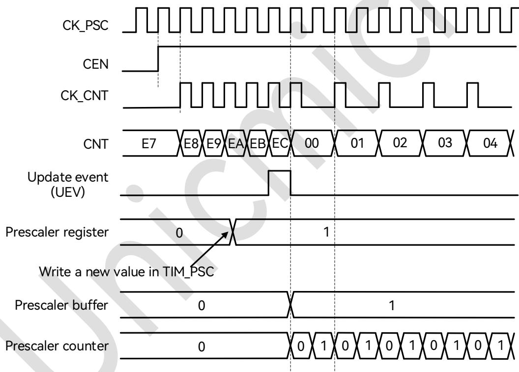
Figure 19-2: Counter Timing Diagram with Prescaler Division Changing from 1 to 2
