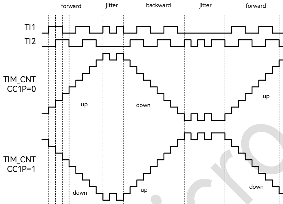
Figure 18-38: Example of Counter Operation in Encoder Interface Mode
