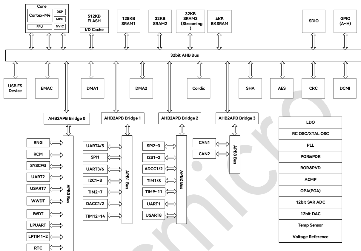
Figure 3-1: Bus Architecture Diagram
