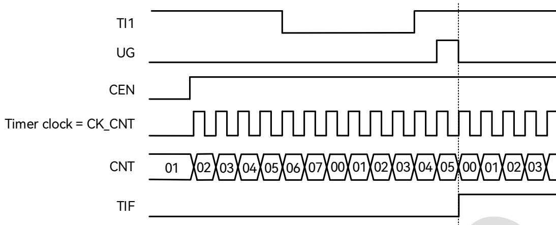
Figure 19-33: Timing Diagram in Reset Mode
