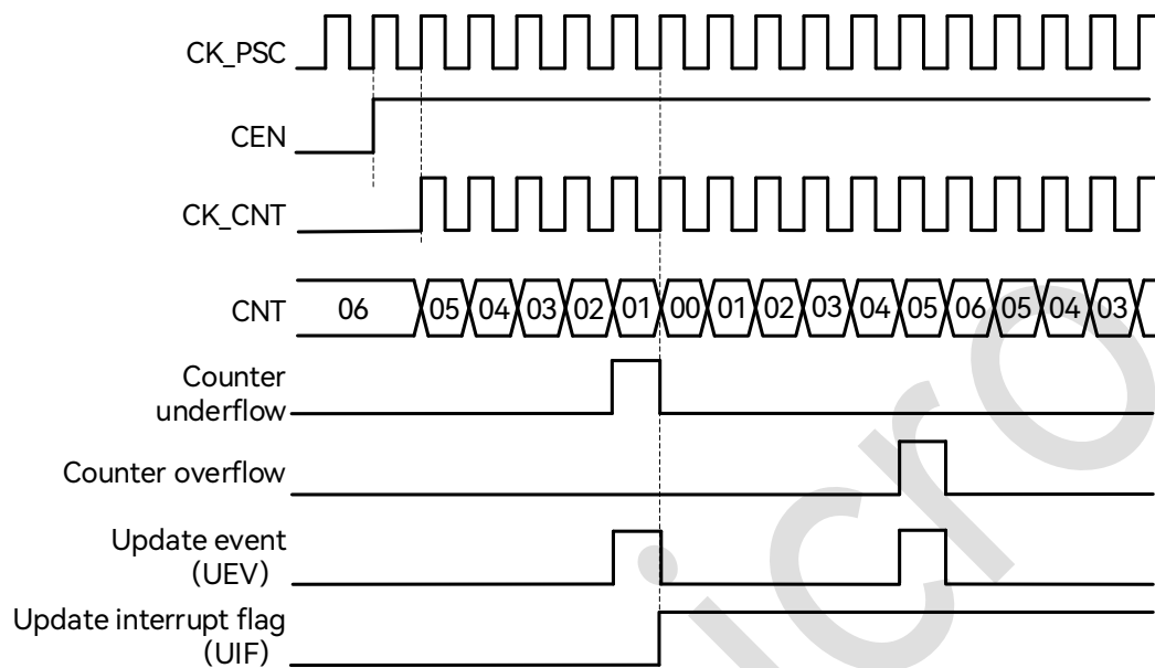
Figure 19-12: Center-aligned Counter Timing Diagram, TIM_PCS = 0, TIM_ARR = 0x6
