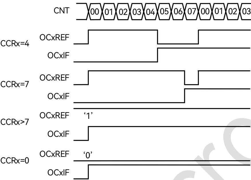
Figure 18-29: Edge-aligned PWM Waveform (ARR = 7)
