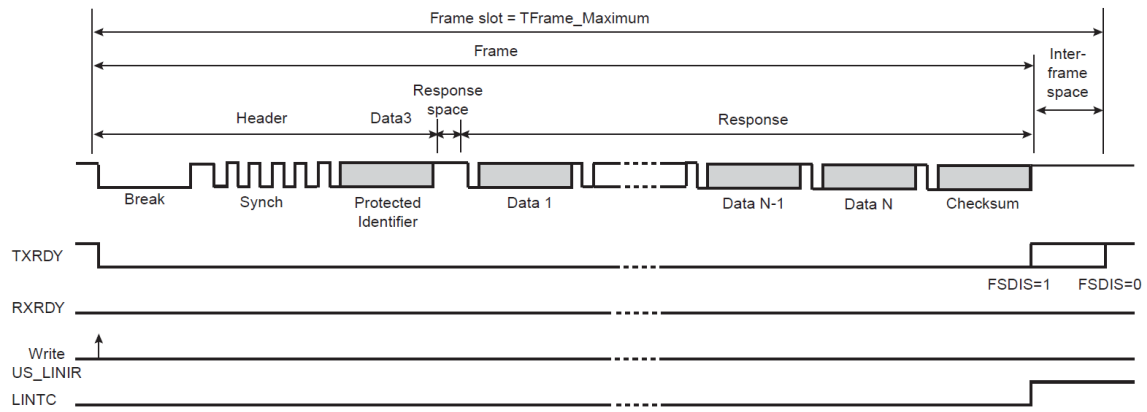
Figure 30-37: Master Node Configuration, NACT = IGNORE
