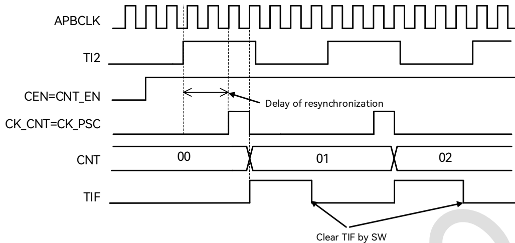
Figure 19-17: Timing Diagram in External Clock Source Mode 1
