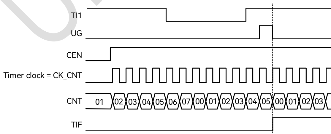
Figure 18-39: Timing Diagram in Reset Mode
