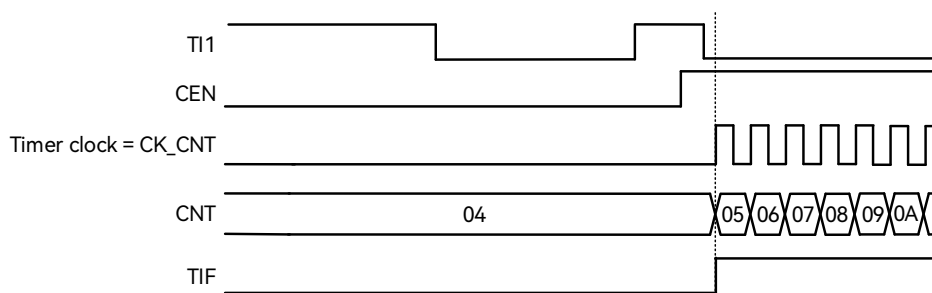
Figure 19-35: Timing Diagram in Trigger Mode
