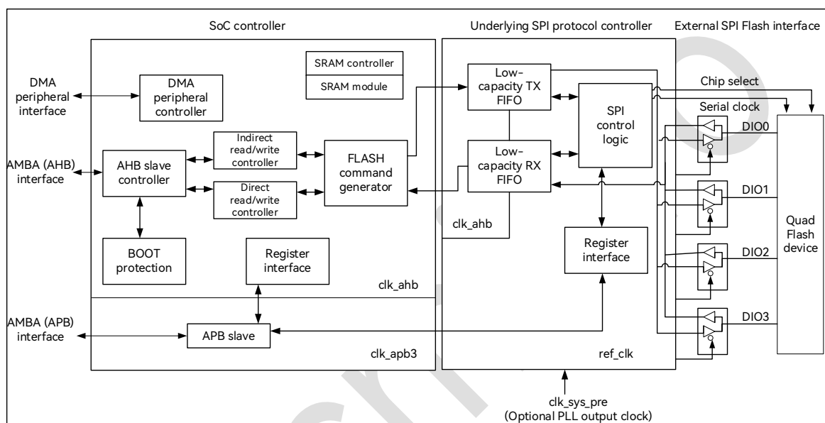
Figure 32-1: QSPI System Block Diagram
