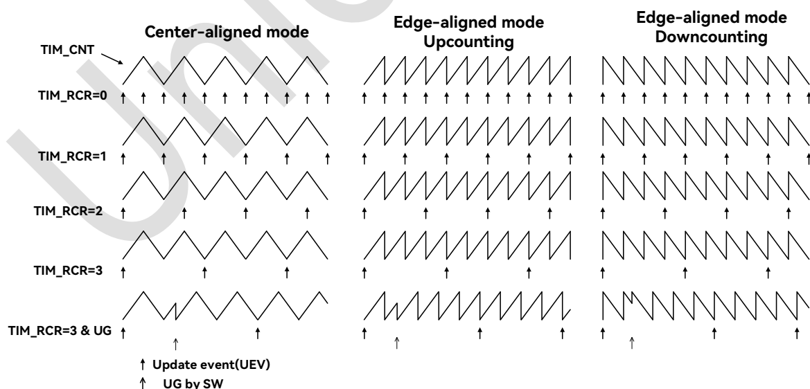
Figure 18-15: Examples of Updating Rate in Different Modes and TIM_RCR Register Setting
