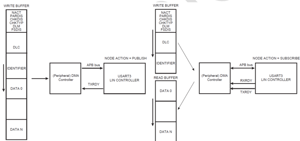
Figure 30-41: Master Node with DMA/PDC (PDCM = 1)
