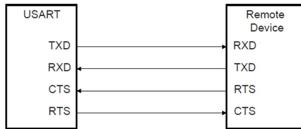
Figure 30-21: Hardware Handshake with Remote Devices
