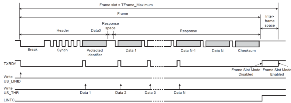
Figure 30-34: USART Frame Slot Mode
