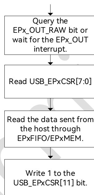
Figure 35-3: USB Endpoint Out Transfer Flowchart
