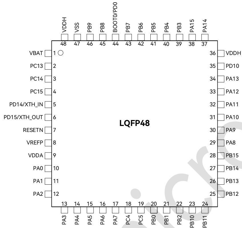
Figure 3-3: LQFP48 (7 * 7 mm) Pinout Diagram
