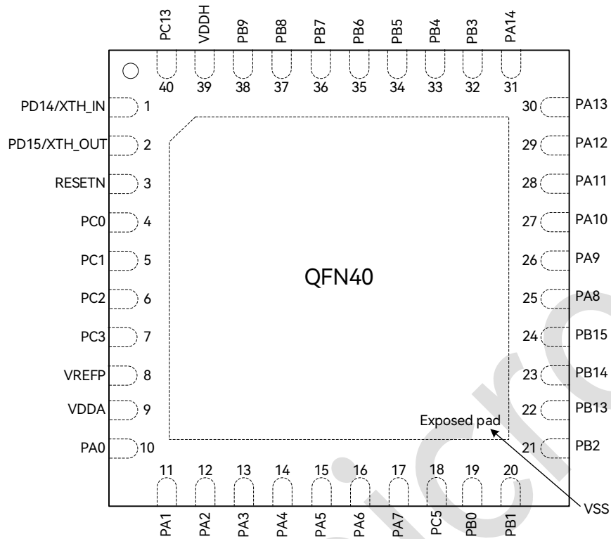
Figure 3-5: QFN40 (5 * 5 mm) Pinout Diagram
