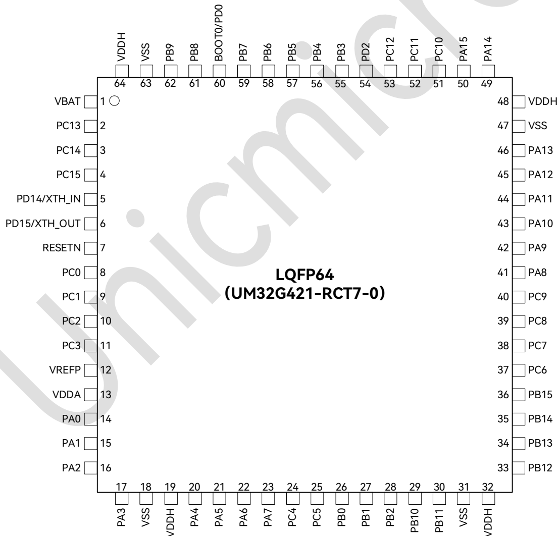
Figure 3-1: LQFP64 (10 * 10 mm) Pinout Diagram
