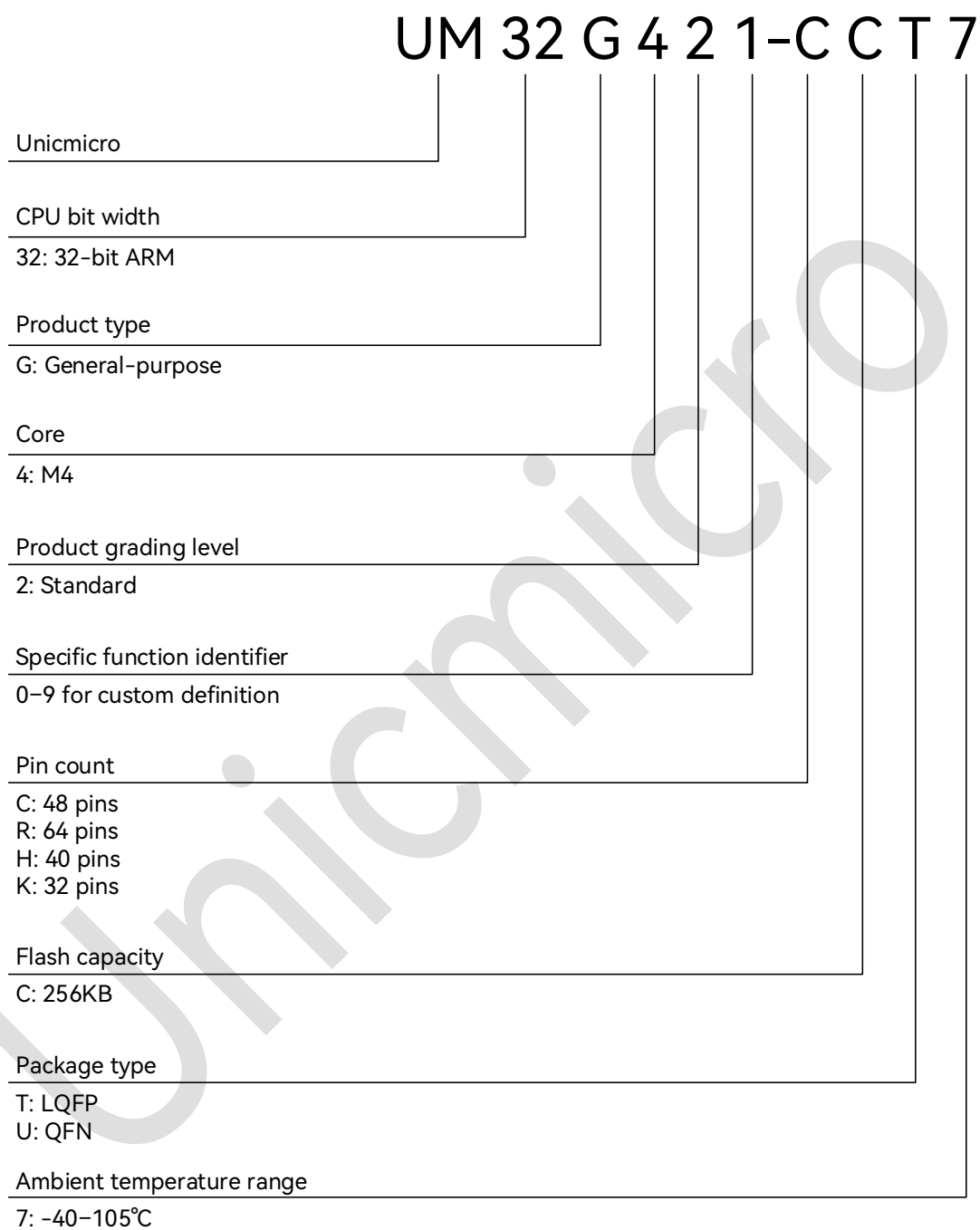
Figure 1-2: Schematic Diagram of Naming Convention
