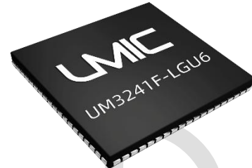
QFN76 (9 * 9 mm)
