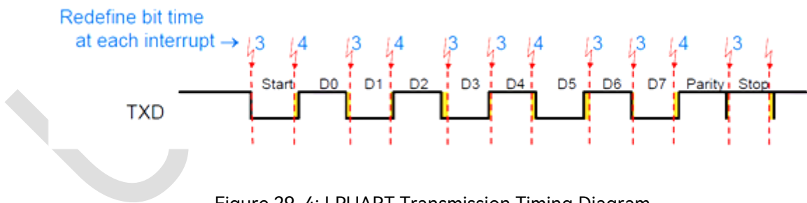
Figure 29-4: LPUART Transmission Timing Diagram
