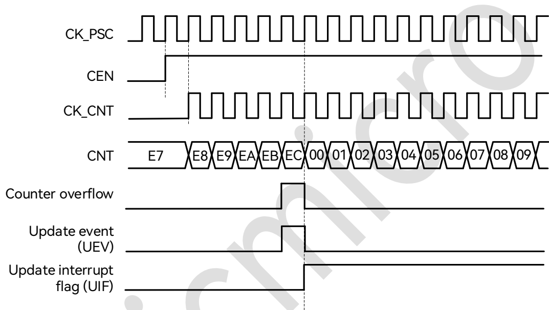
Figure 19-4: Up-counting Waveform Diagram, Internal Clock not Divided
