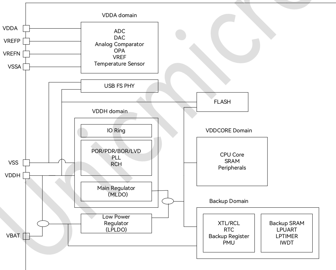
Figure 5-1: System Power Supply Scheme
