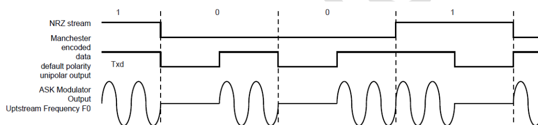
Figure 30-13: ASK Modulator Output
