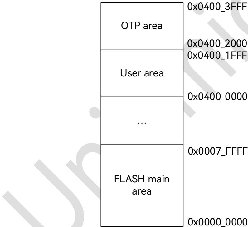
Figure 4-1: EFC Memory Address Mapping
