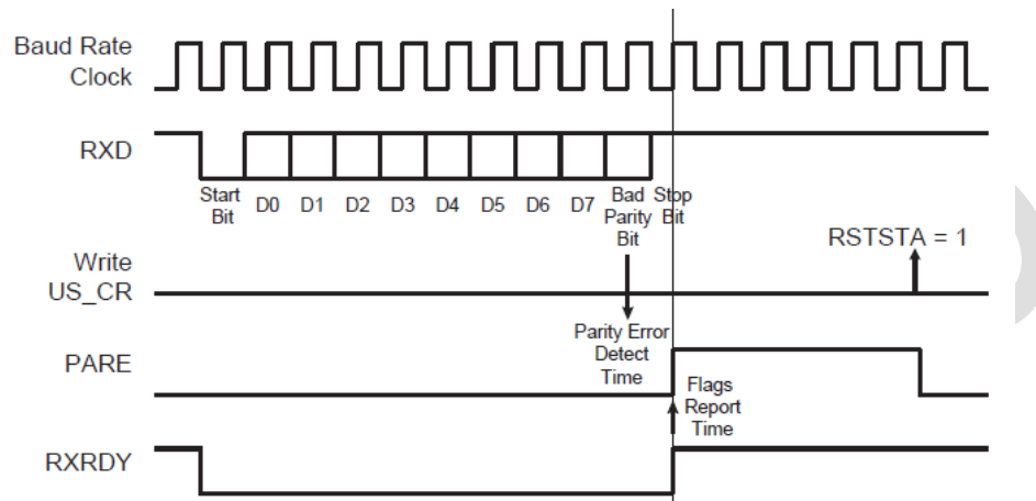
Figure 30-17: Parity Error Timing Diagram
