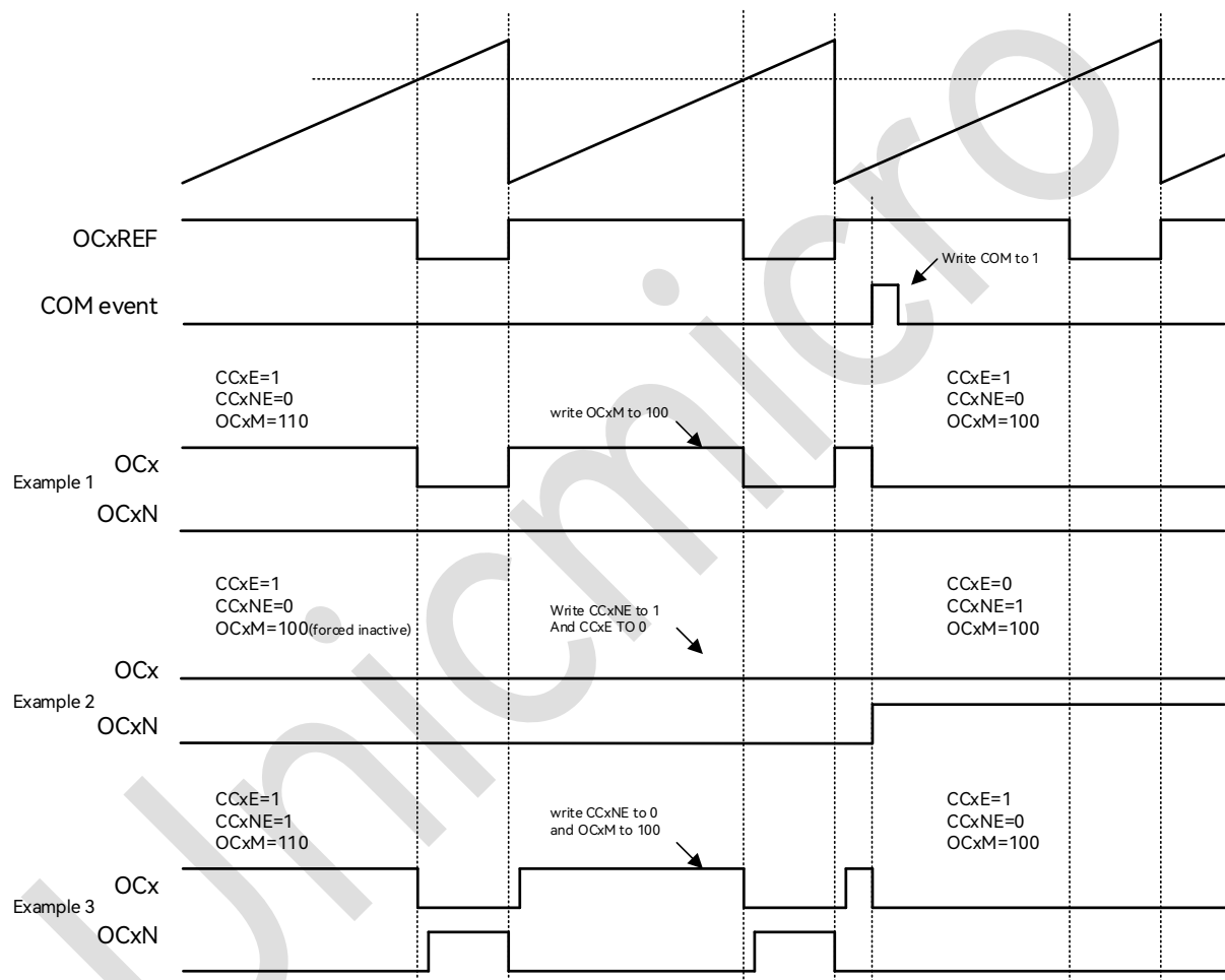
Figure 18-35: 6-step PWM Generation, COM Example (OSSR = 1)
