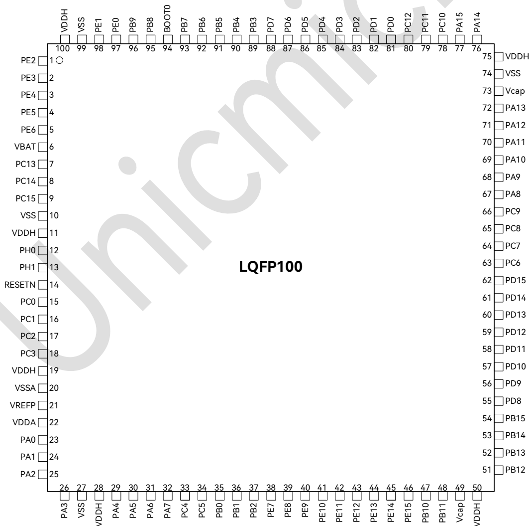
Figure 3-1: LQFP100 Pinout Diagram
