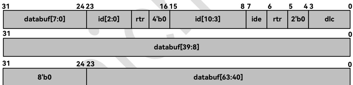
CAN Rx Fifo for 11bits ID
