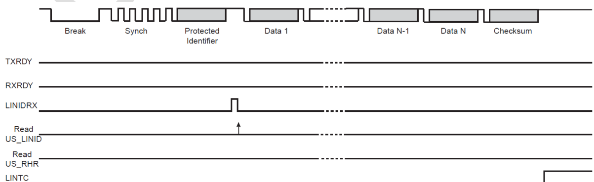
Figure 31-37: Slave Node Configuration, NACT = IGNORE
