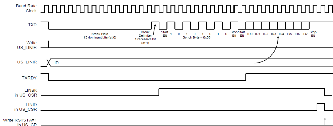
Figure 31-26: Message Transmission
