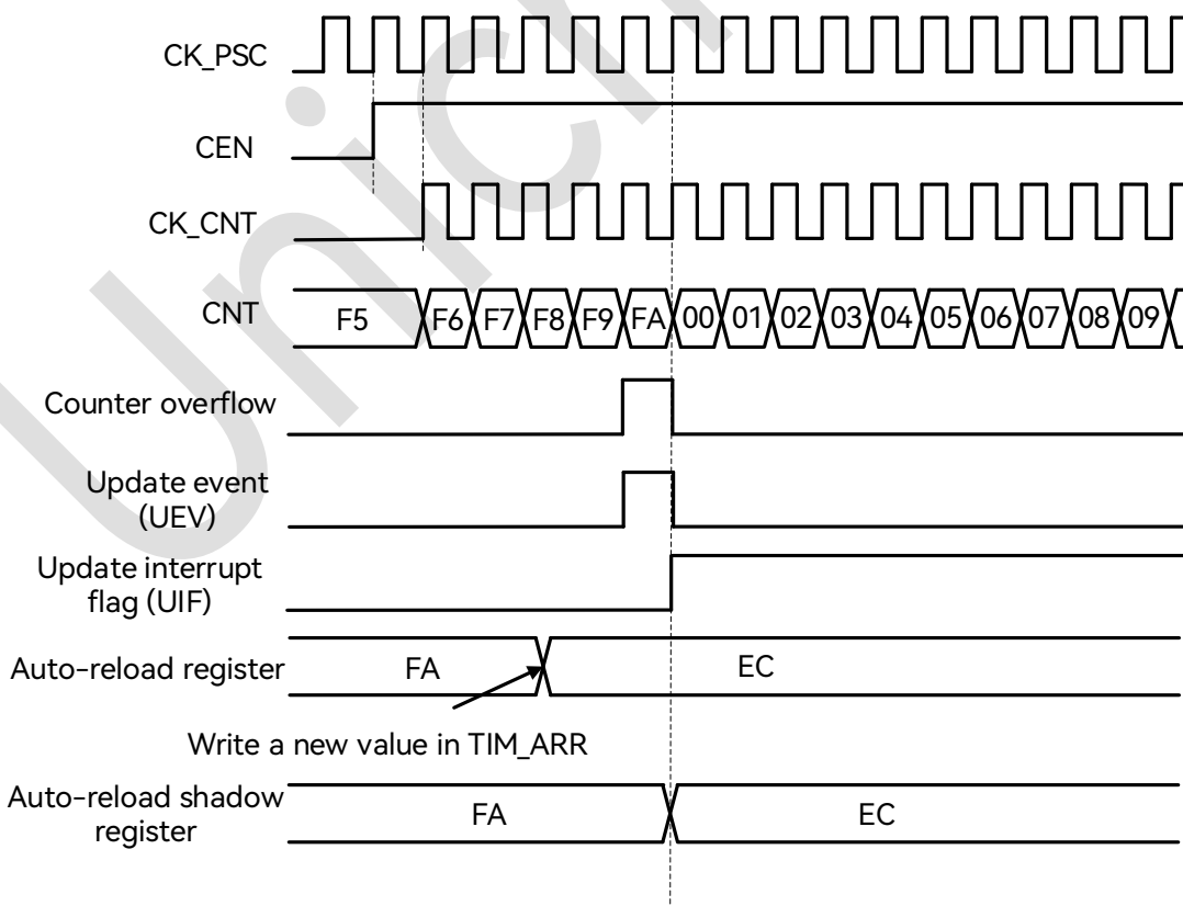
Figure 16-7: Counter Timing Diagram, Update Event when ARPE = 1 (TIM_ARR Preloaded)
