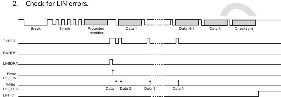
Figure 31-35: Slave Node Configuration, NACT = PUBLISH
