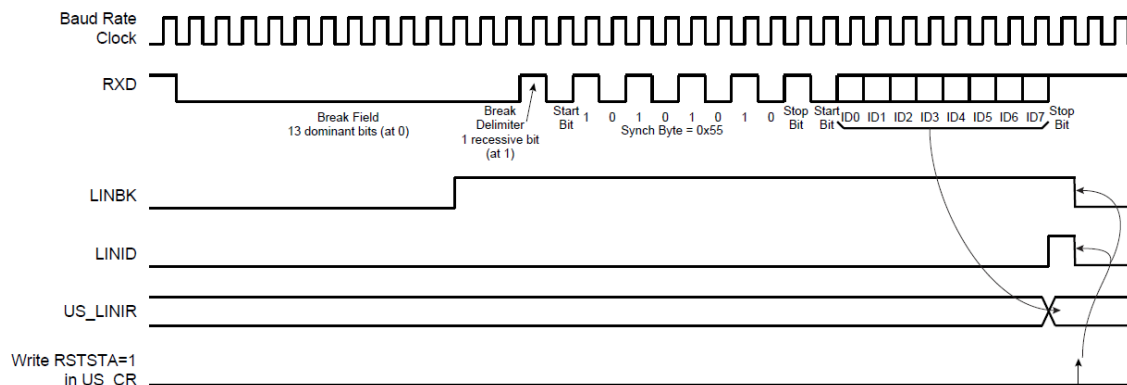
Figure 31-27: Message Reception
