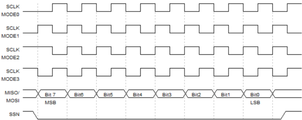
Figure 33-4: Transmission Timing Diagram of SPI in Different Modes in Motorola Mode
