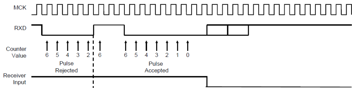
Figure 31-23: IrDA Demodulator Operation
