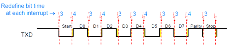
Figure 30-4: LPUART Transmission Timing Diagram
