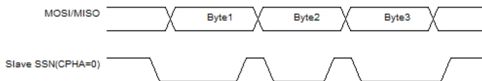
Figure 32-3: SPI SSN Timing Diagram ( CPHA = 0 )
