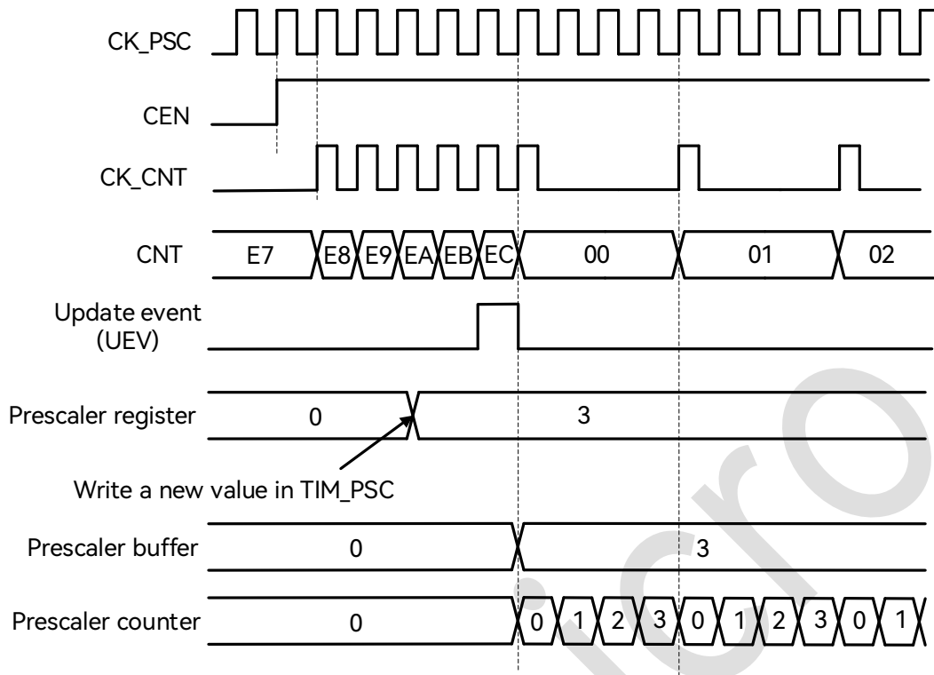
Figure 16-3: Counter Timing Diagram with Prescaler Division Changing from 1 to 4
