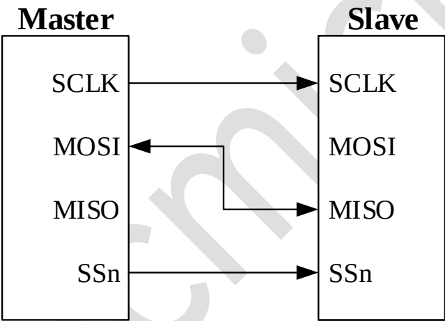
Figure 32-7: Half-duplex Communication
