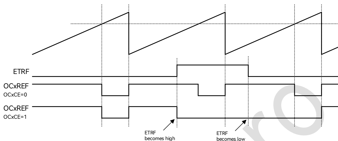
Figure 17-31: ETRF Signal Clearing OCxREF of TIM
