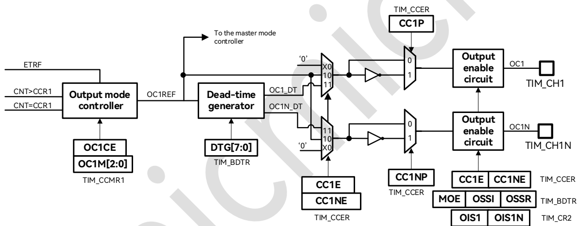
Figure 17-23: Capture/Compare Channel 1 Main Circuit
