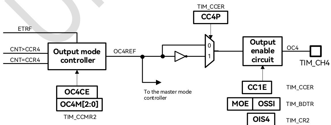
Figure 17-25: Output Stage of Capture/Compare Channel (Channel 4)
