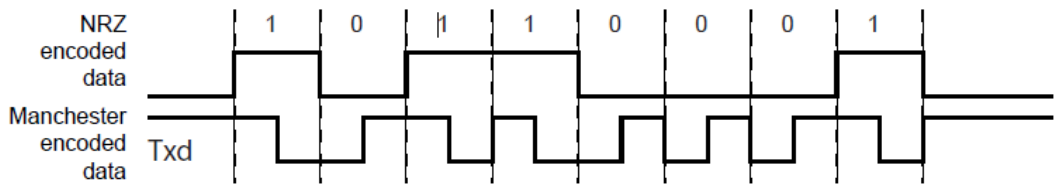
Figure 31-3: NRZ Code to Manchester Code
