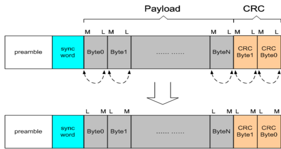
图 7-5: PAYLOAD_BIT_ORDER 操作
